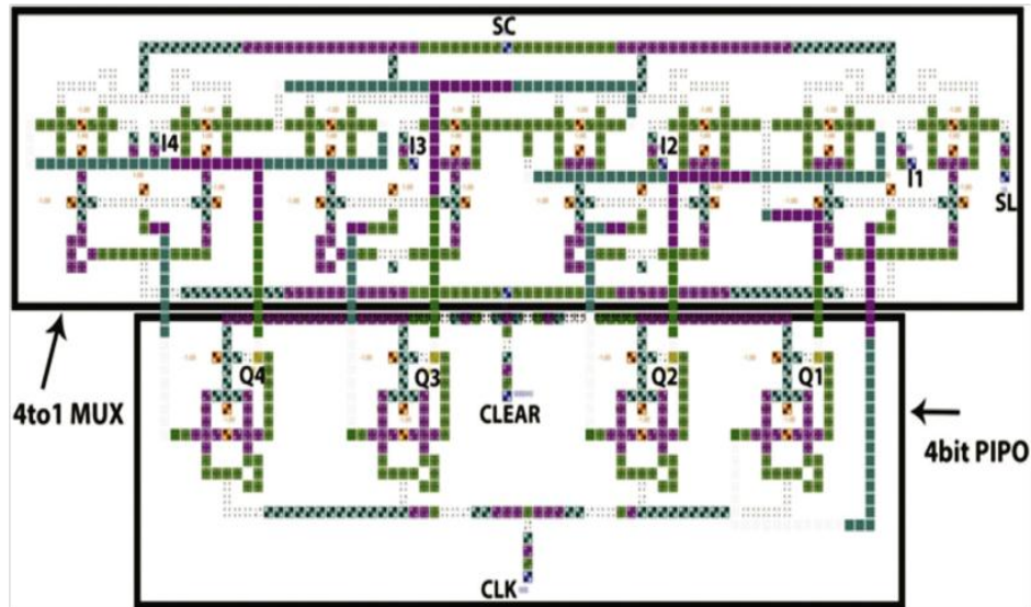
Figure 10. Proposed Circuit (Universal Shift) PIPO-4-Bit.
