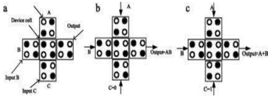
Figure 5. Logic Gates using QCA. Source: (Ganesh EN, et al).
