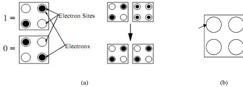
Figure 1. (a) QCA (b) Single Cell. Source: (Sabbaghi-Nadooshan, et al).
