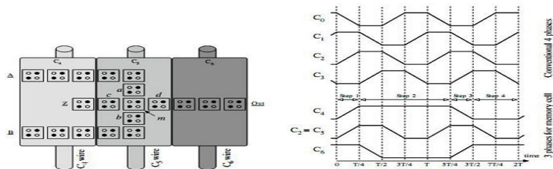
Figure 5. Line based QCA Memory. Source: (Walus K, et al).
