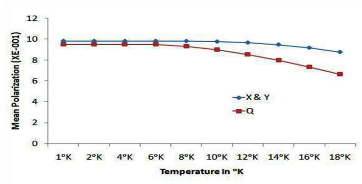
Figure 17. Comparison of the Proposed Model with Reference Model in terms of Temperature .
