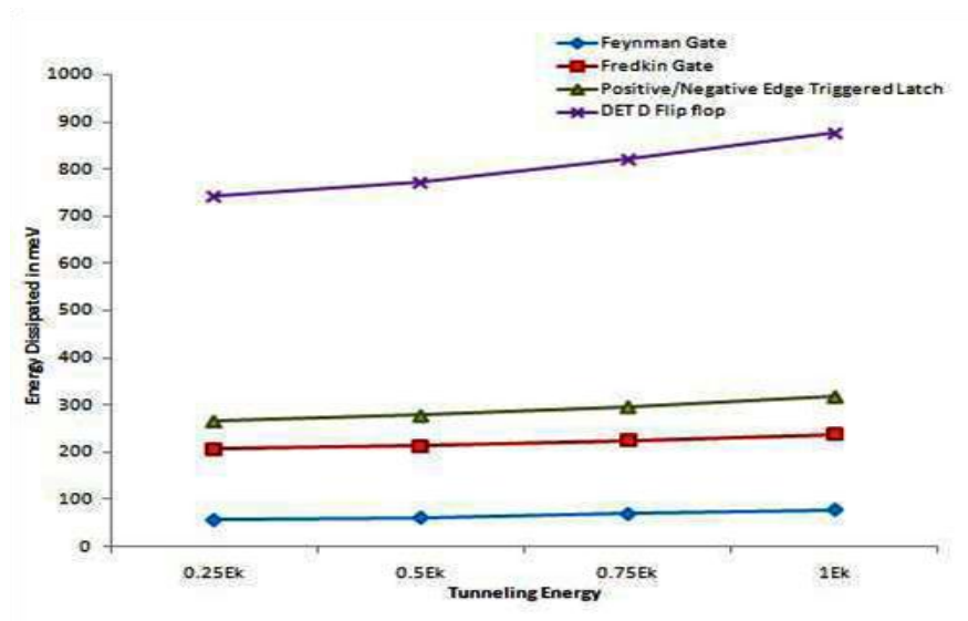
Figure 16. Power & Energy Analysis of the Proposed Model.
