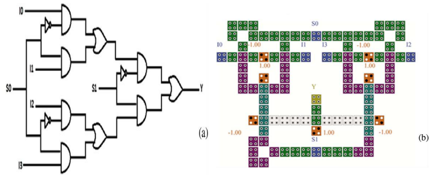
Figure 14. Schematic Circuit & QCA Implementation of 4: 1 MUX used in Proposed Circuit.
