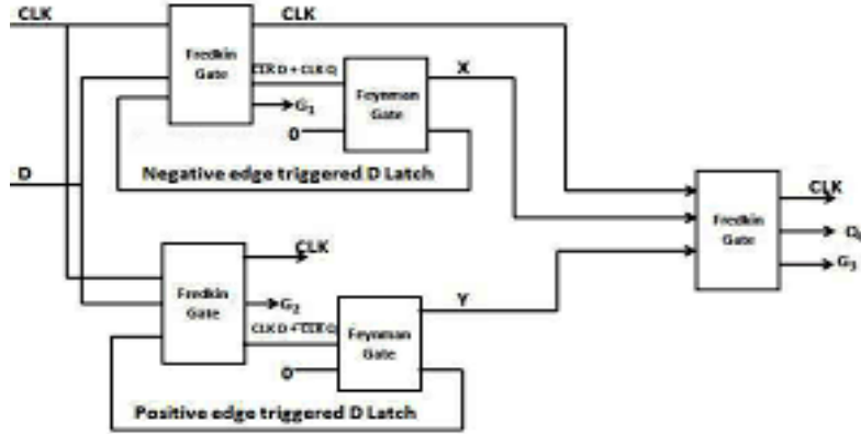
Figure 9. Basic Diagram of Shift Register Memory. Source: (H. Thapliyal, et al).
