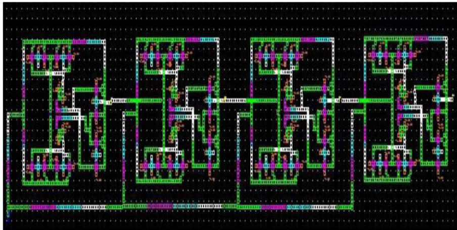
Figure 12. Proposed Circuit (Universal Shift) SIPO 4-Bit.
