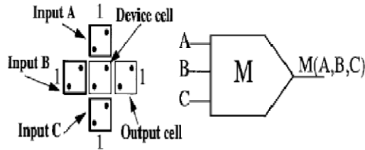
Figure 4. M-Gate. Source: (Shamsabadi AS, et al).
