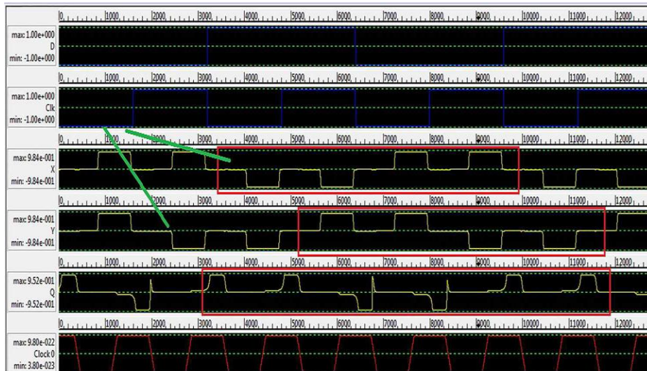
Figure 15. Simulation results of the Proposed Circuit using QCA Designer Tool.
