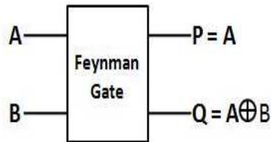
Figure 7. Feynman Gate.
