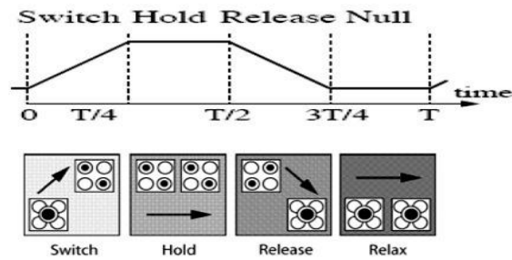
Figure 2. QCA Clockwise Sequencing. Source: (Liu W , et al).
