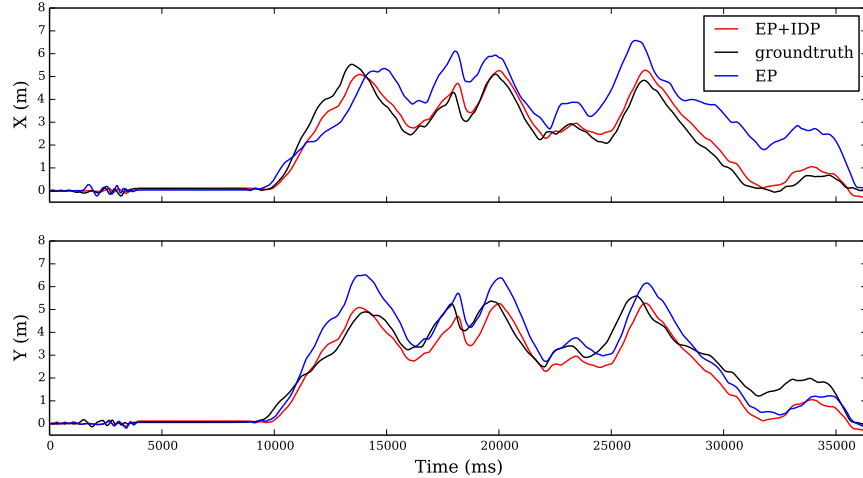
Figure 4: The obtained results of the proposed hybrid technique. Normal estimated position, EP in the figure, and the combination of inverse-depth mapping and EP, i.e., EP+IDP , are compared against the real position of the camera, i.e., the groundtruth
