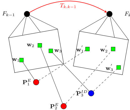
Figure 2: An example of Euclidean points that are shown in red and inverse depth points that are shown in blue for two consecutive frames. A direct method is applied to obtain the transformation matrix, i.e., T_{k,k-1} , by minimizing the photometric error of the patches that are shown in green squares in the figure. As can be seen, the method uses both Euclidean and inverse-depth points
