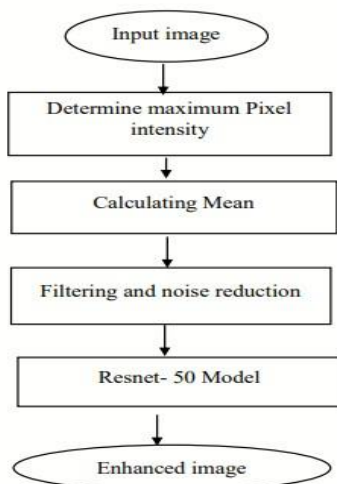
Fig-4: Flow Chart of Image Enhancement Using Resnet50
