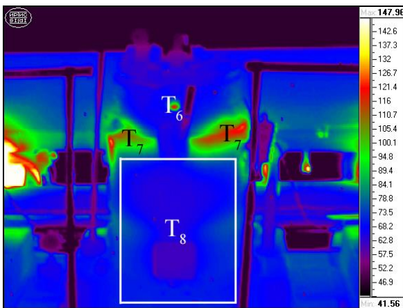
Fig. 2. Power Cylinder (10 units per plant)
