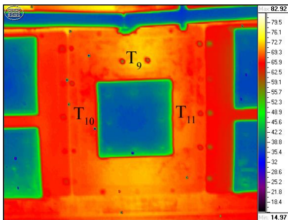
Fig. 3. Housing Assembly fragment in the Connecting-Rod Gear area (5 units per plant)
