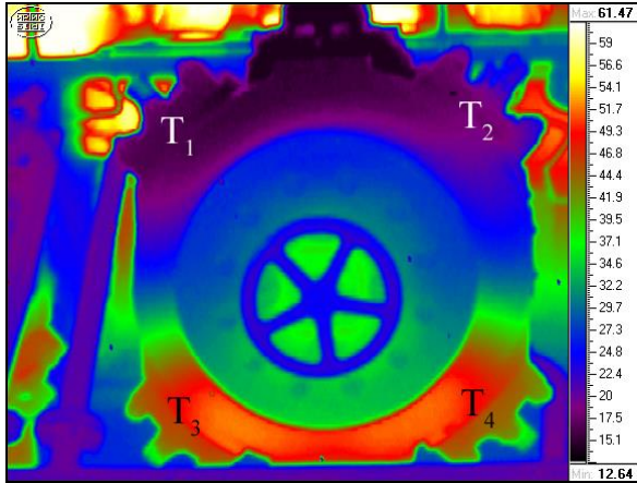
Fig. 1. Compressor Cylinder (5 units per plant)
