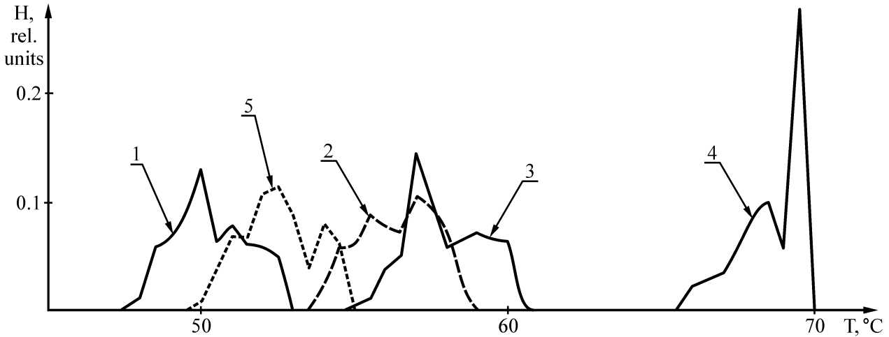
Fig.4. Histograms envelopes for a group (5 units) of pressure valves that belong to one gas engine compressor plant
