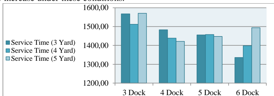
Figure 7. Service Time Comparison Chart
