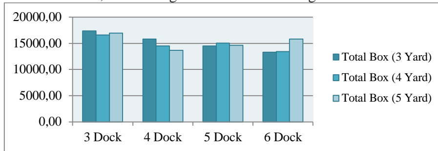
Figure 6. Total Box Comparison Chart
