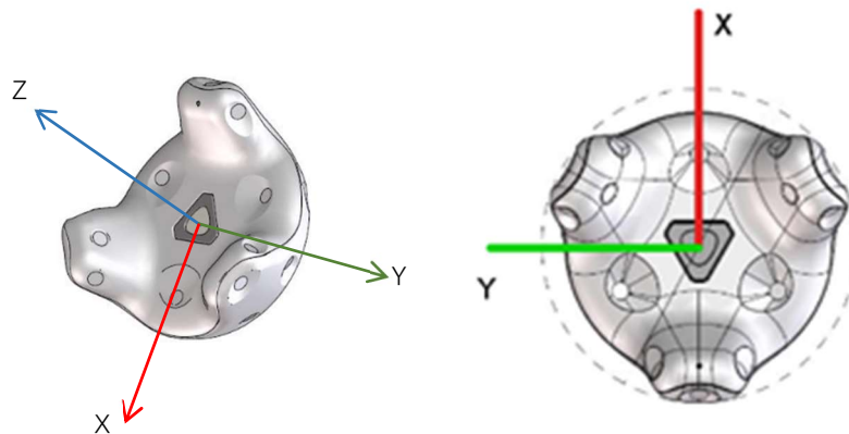
Figure 4. Vive Tracker's coordinate system
