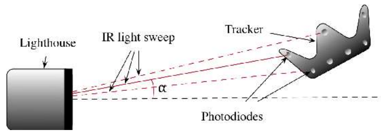
Figure 2. Positioning principle of Lighthouse technology
