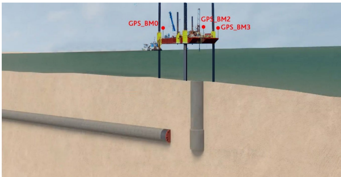
Figure 3: PVC pipe installation from the Barge
