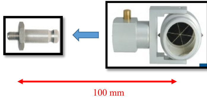
Figure 5: Tunnel Control Point
