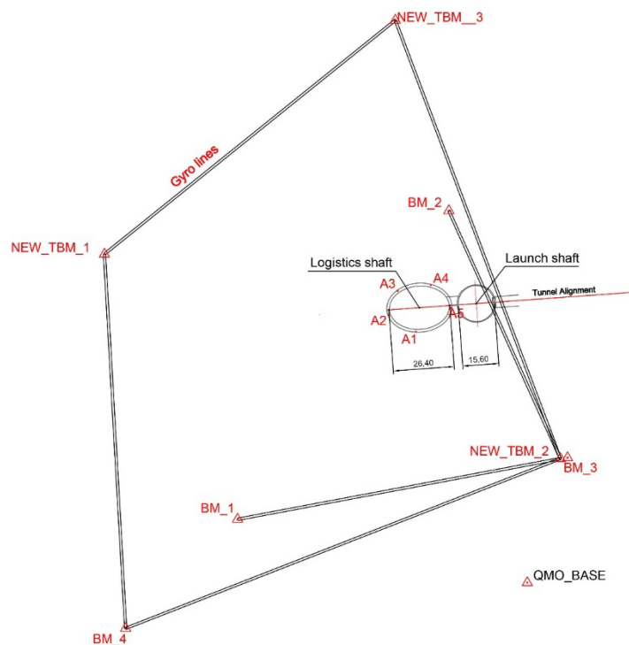
Figure 2. Control points of the First and Second levels
