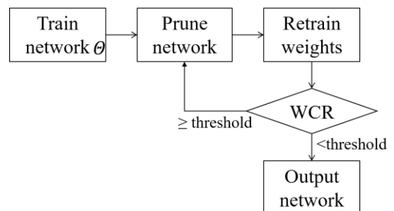
Fig. 2 Block diagram of the iterative pruning method with retraining.
