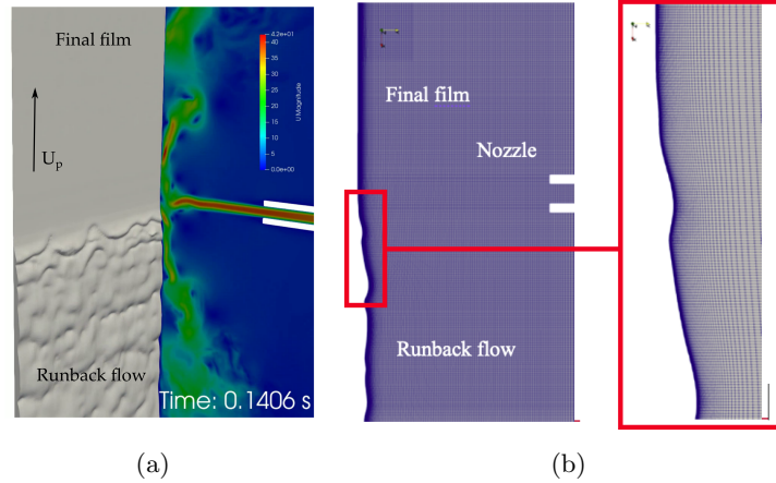
Figure 1: 3D view of the jet wiping process (a), and snapshot of the mesh deformation in this approach where the liquid film is replaced by a solid wall (b).
